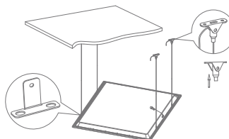
2. Hang the panel to ceiling with suspended installation kits.
