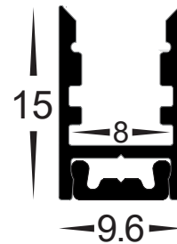
Aluminium Channel Dimensions
