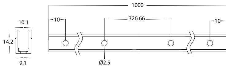
PVC Channel Dimensions
