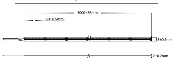
LED Strip Dimensions
