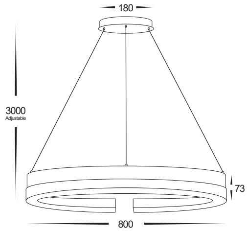
HV6094T Dimensions
