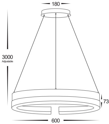
HV6092T Dimensions
