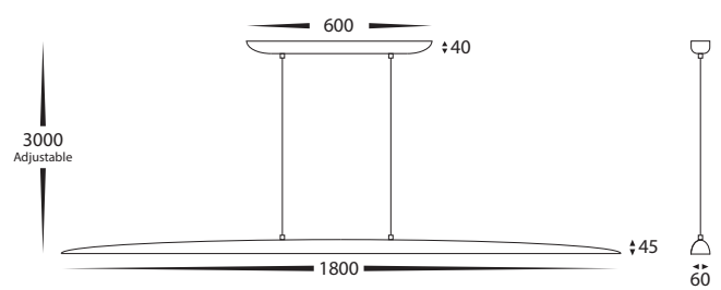
HV6012T Dimensions
