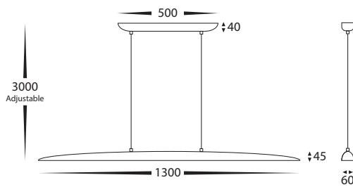
HV6010T Dimensions
