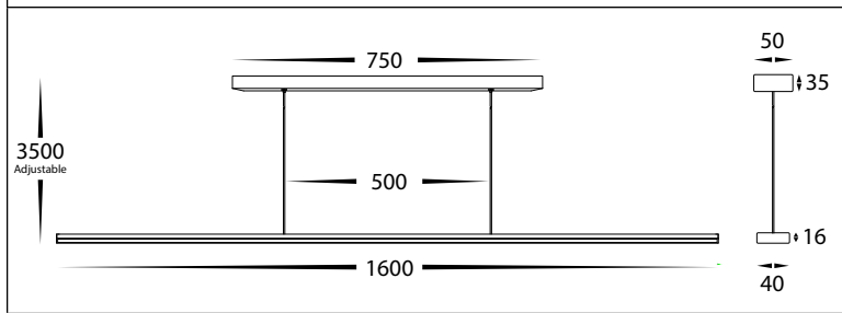
HV6006T Dimensions
