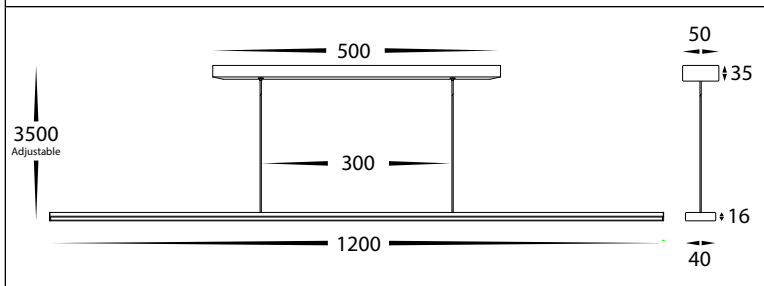
HV6005T Dimensions
