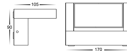
HV3731T-BLK Dimensions
