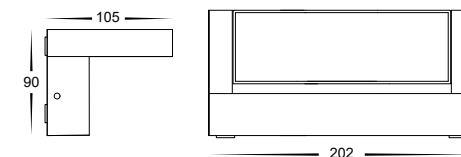
HV3733T-BLK Dimensions
