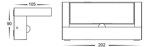
HV3732T-BLK-PIR Dimensions
