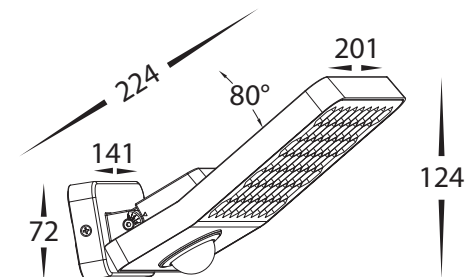
HV3722N-GRY Dimensions
