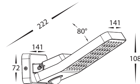
HV3721N-GRY Dimensions
