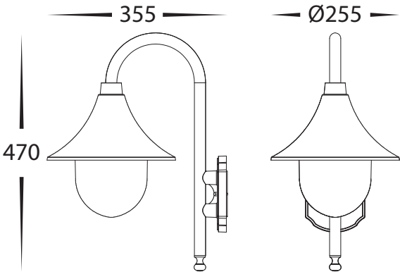
HV3554W Dimensions
