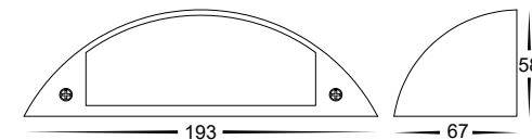
Dimensions for HV3253
