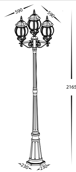
HV1673W-BLK Dimensions
