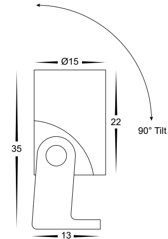
Surface Mounted Dimensions
