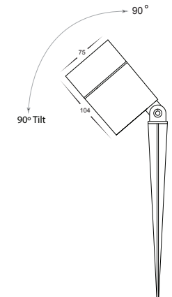
HV1429T-12W Dimensions
