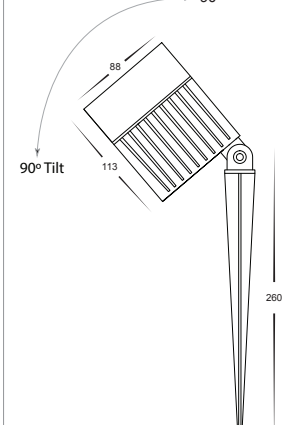
HV1429T-24W Dimensions
