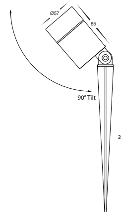
HV1429T-7W Dimensions
