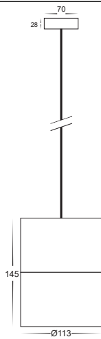
HCP-8921204-PDT + HCP-8931204-PDT Dimensions
