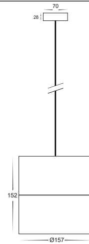
HCP-8921804-PDT + HCP-8931804-PDT Dimensions
