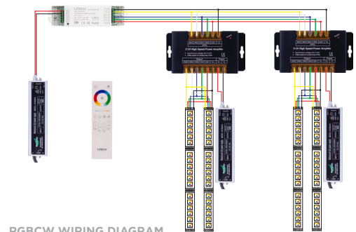
RGBCW WIRING DIAGRAM
