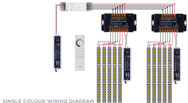
SINGLE COLOUR WIRING DIAGRAM
