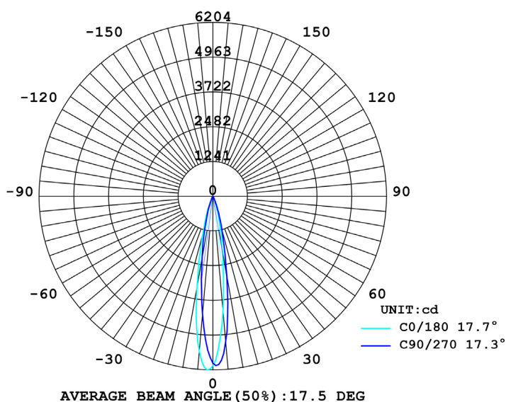
PHOTOMETRICS
