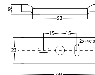
Mounting Base
