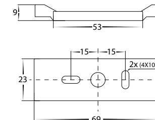
Mounting Base
