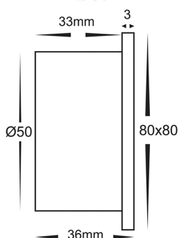
Cutout without Canister Ø60
