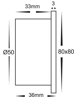
Cutout without Canister Ø60
