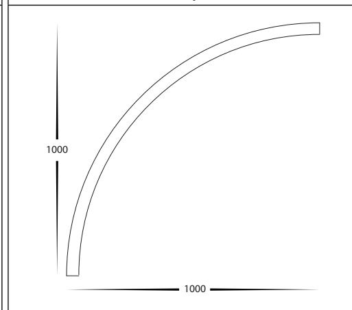
HCP-6923235-2-1/4 Dimensions
