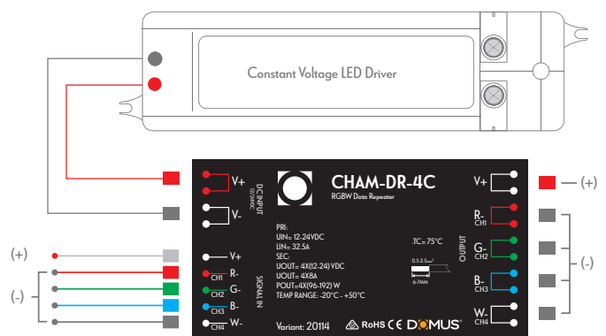
Single Colour Dimming Expansion (Fig 2)
