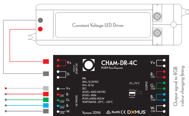
RGBW Colour Changing (Fig 1)
