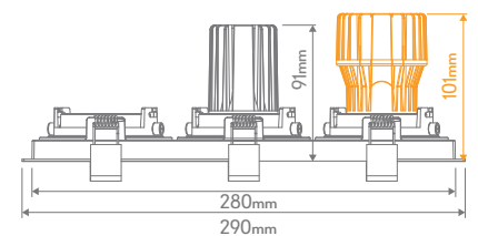
Cutout: L280mm x W100mm
