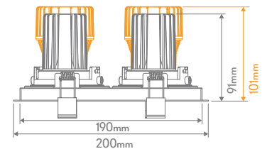
Cutout: L190mm x W100mm
